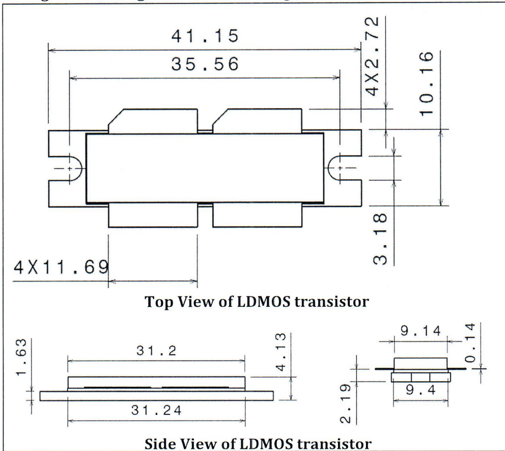
Image-1: Drawing No 1: Case drawing for LDMOS transistor
