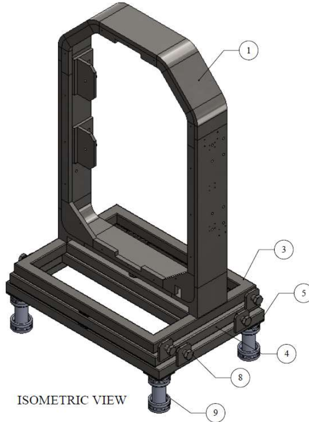
Fig 1: Beam Source Frame Structure
